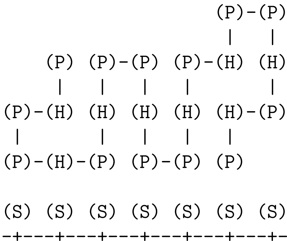
Figure 3: Lowest energy conformation of S_{21} on a weakly attractive surface. For surface interaction \epsilon_S = 0.08 , E = -7.48
