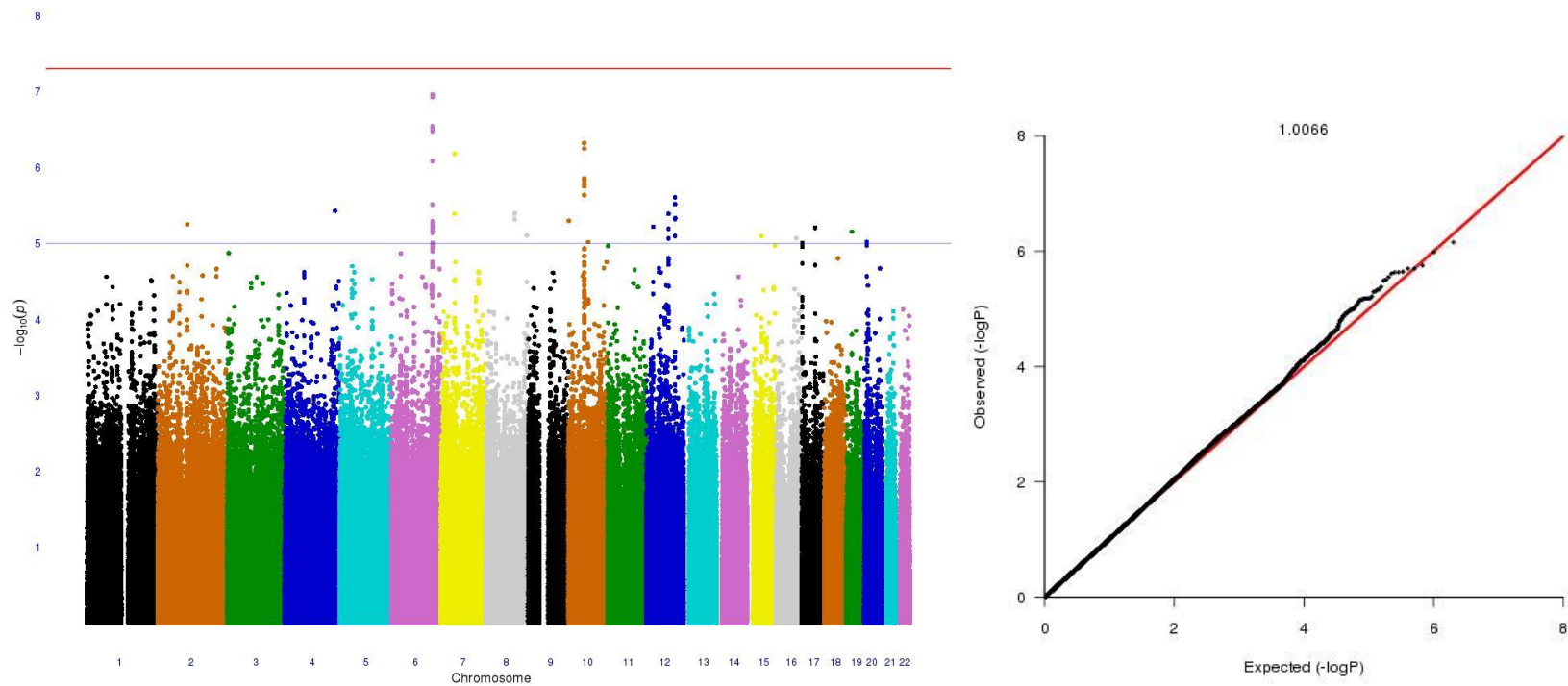
Figure 2.5.3 Manhattan and QQ plots of GWAS results for glucose responses to HCTZ in African-America 94
