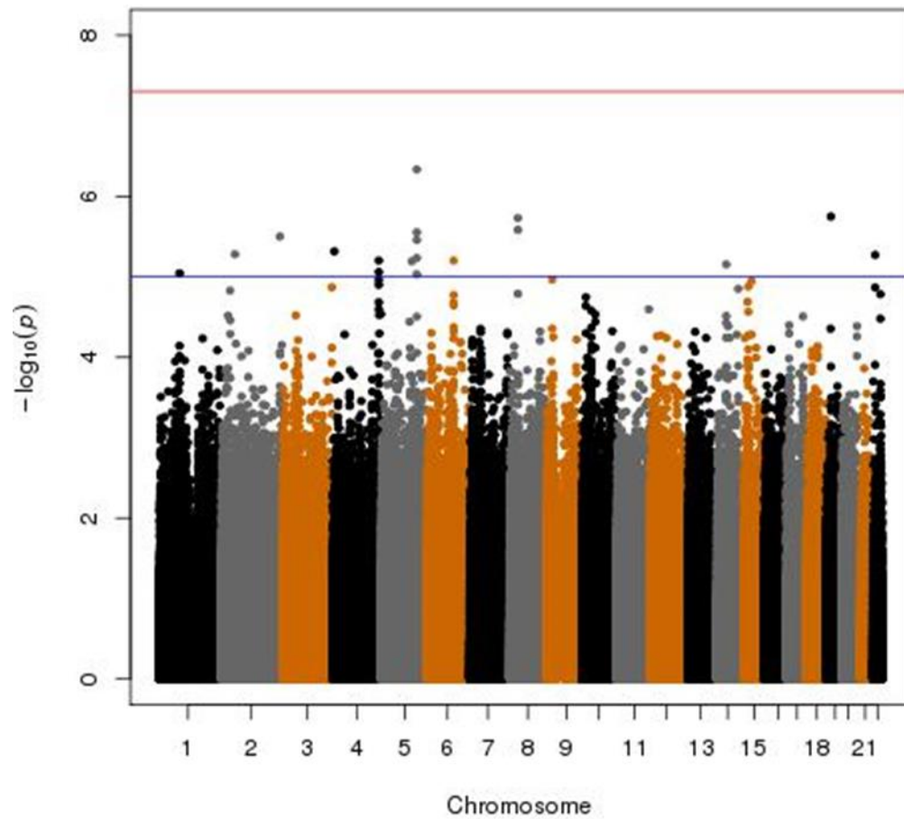
Figure 3.3.2 Manhattan and Q-Q plots of Thiazide SNP interaction estimates for fasting insulin after the meta-analysis from 12 cohorts of European ancestry.
