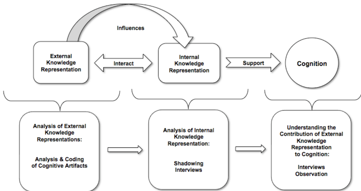
Figure 2: Methodology Framework
