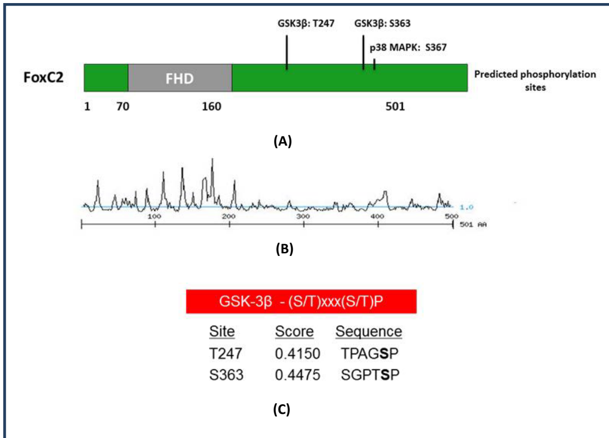
Fig. 1. Potential phosphorylation sites prediction for FOXC2 using Scansite Motif Scan analysis program. A) Predicted phosphorylation sites for GSK-3β. B) The surface accessibility map for FOXC2. C) The candidate sequence for GSK-3β as well as the location of the potential GSK-3β phosphorylation site within the FOXC2 amino acid sequence.
