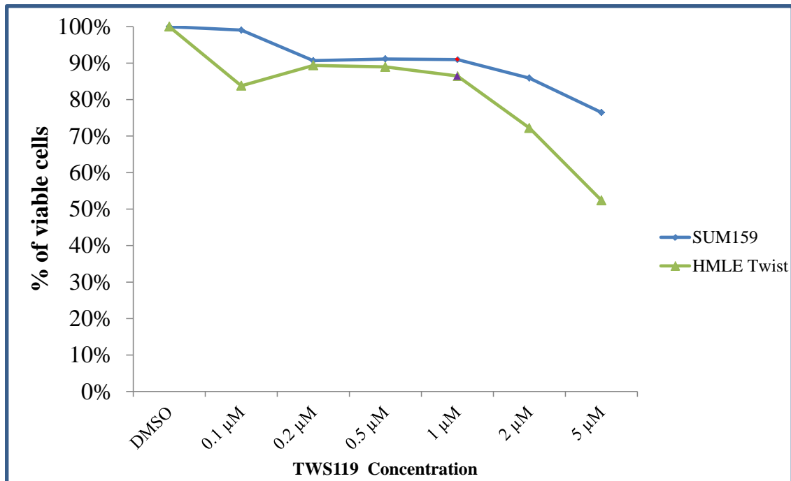
Fig. 4. Cell viability assay using TWS119. Percentage of viable cells after 0.1, 0.2, 0.5, 1, 2, 5 \mu\text{M} of TWS119 exposure for 24 hours using HMLE Twist and SUM159 cells relative to DMSO. FOXC2 mRNA level does not change significantly upon treatment with TWS119.
