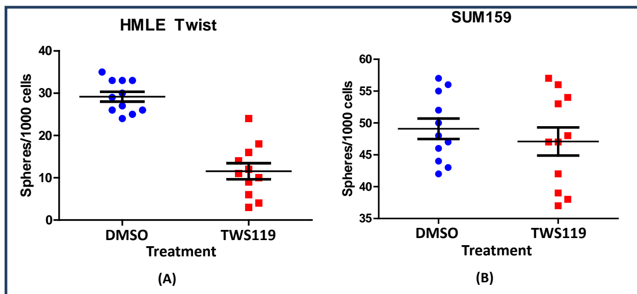
Fig. 10. Decrease in sphere formation in response to TWS119 treatment. HMLE Twist (A) and SUM159 (B) cells plated in low density culture plate and the number of spheres counted after two weeks of culture either presence of DMSO or 1 \mu M TWS119.
