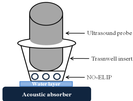
Figure 4.1 Experimental setup for ultrasound-triggered release study (40)
