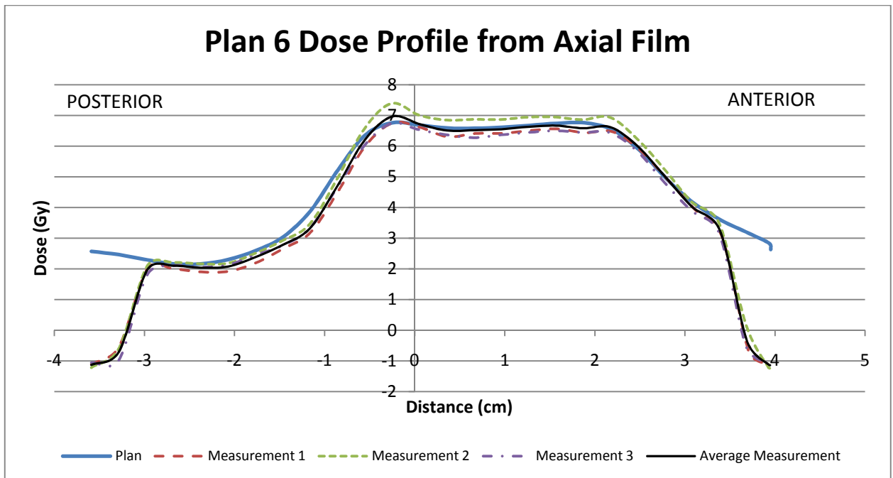
Figure C.16 Posterior-to-anterior dose profile of Plan 6 as planned by the TPS and measured with the three axial films
