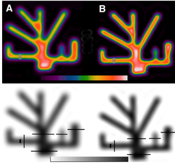
Figure 4. PET images of tree phantom filled with Rb-82 (panel A) and separately with F-18 (panel B), with color scale above and the same images in black on white below. Maximum activity of bar scale for Rb-82 is 184.630 Bq/cc (4.99 \mu Ci/cc) and for F18 is 498,202 Bq/cc (13.46 \mu Ci/cc) for both color and black on white displays. The small rectangular ROI is 1 cm tall in scanner space as size reference corresponding to 1 cm physical width of that phantom branch. The narrower lines indicate the path of the ROI of 0.85 mm radius stepped across the phantom branches in 0.85 mm increments for measuring profiles of quantitative activity.
