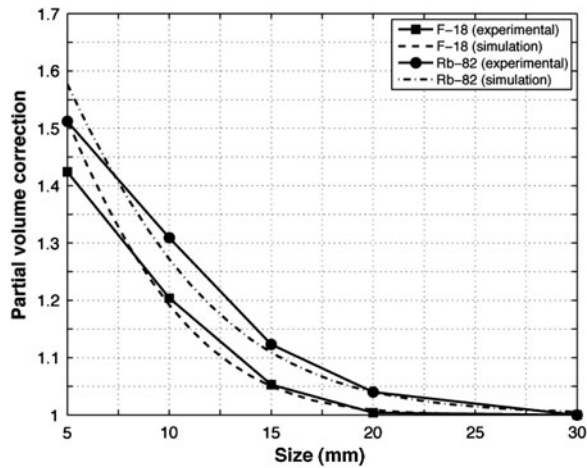
Figure 6. Partial volume corrections based on peak PET measured activity across each phantom dimension as a ratio to true peak activity for Rb-82 and F-18. The dashed lines indicate the theoretical curves derived from the simulation illustrated in Figure 1.
