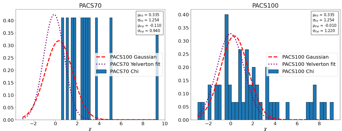
Fig. 2. Histograms of excess significance for PACS70 (left) and PACS100 (right) measurements. The purple dotted curve shows the noise distribution derived by Yelverton et al. (2019) for their PACS70 (left) and PACS100 (right) data sets, while the red dashed curve shows the same noise distribution derived from our PACS100 data set—our PACS70 data set was not large enough to robustly fit the noise distribution. The values noted as \mu_{\text{Fit}} and \sigma_{\text{Fit}} are respectively the mean and standard deviation of the significance in our PACS100 distribution, while \mu_{\text{Yel}} and \sigma_{\text{Yel}} are the ones from Yelverton et al. (2019).
