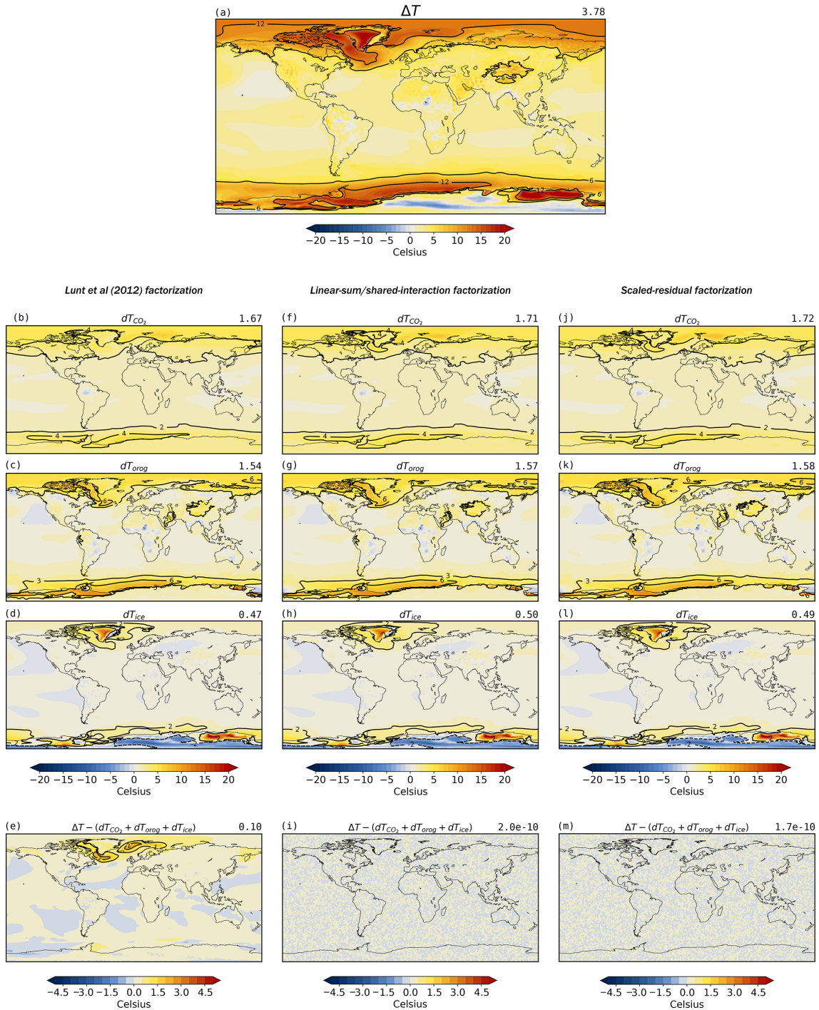
Figure 4. Comparison of various factorisation methods. (a) The mid-Pliocene minus pre-industrial anomaly ( T_{111} - T_{000} ) modelled by Chandan and Peltier (2017). (b–m) The top three rows present factorisations of the total anomaly into contributions arising from changes to CO_2 (upper, b, f, j), orography (middle, c, g, k), and ice sheets (lower, d, h, l), while the bottom row shows the residual required for completeness (e, i, m). Note that the residual term, R , for panel (e) is given by Eq. (14) and is equal to T_{111} - T_{000} - (\Delta T'_{CO_2} + \Delta T'_{orog} + \Delta T'_{ice}) . The first column (b, c, d, e) shows results using the methodology of Lunt et al. (2012) and is identical to results reported in Fig. 7 of Chandan and Peltier (2018). The second column (f, g, h, i) shows results from the linear-sum/shared-interaction factorisation (Eq. 6), and the third column (j, k, l, m) shows results of the scaled-residual factorisation (Eq. 15). The values at the top-right of each panel give the global mean, in units of °C.
