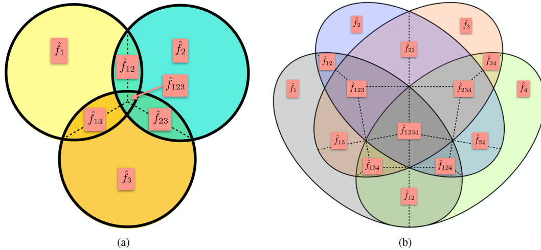
Figure 3. (a) Visual representation of the shared-interaction factorisation for N = 3 , as given by Eq. (10). The straight dotted lines represent the sharing of the interactions according to Eq. (11). (b) Visual representation of the shared-interaction factorisation for N = 4 . The straight dotted lines represent the sharing of the interactions according to Eq. (13).
