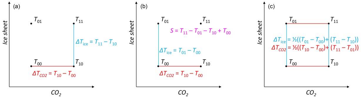
Figure 1. Three different factorisation methods of temperature, T , for two variables ( \text{CO}_2 and ice sheets). (a) Linear factorisation, (b) Stein and Alpert (1993) factorisation, (c) Lunt et al. (2012) factorisation. The temperature, T , can be considered as a surface in a third dimension sitting above the two-dimensional plane of \text{CO}_2 and ice sheets. In Eqs. (1), (3), and (4), \Delta T_1 = \Delta T_{\text{CO}_2} and \Delta T_2 = \Delta T_{\text{ice}} .
