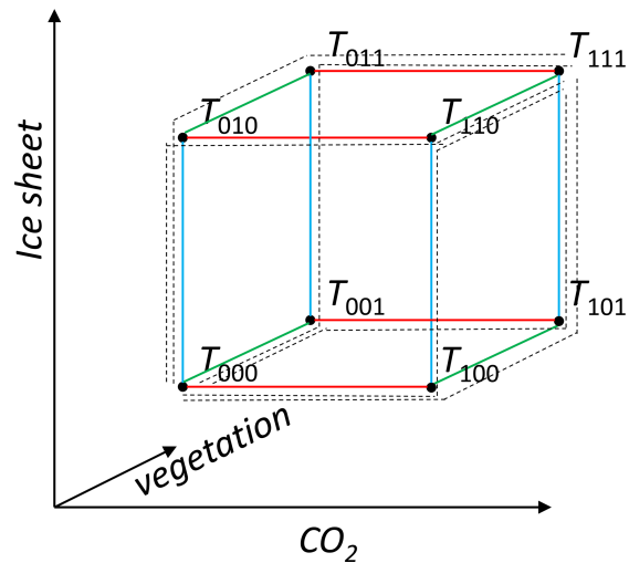
Figure 2. Simulations and linear factorisations in an N = 3 factorisation. Edges that represent changes in \text{CO}_2 are in red, changes in ice are in blue, and changes in vegetation are in green. The paths associated with all three possible linear factorisations are shown with dotted lines.
