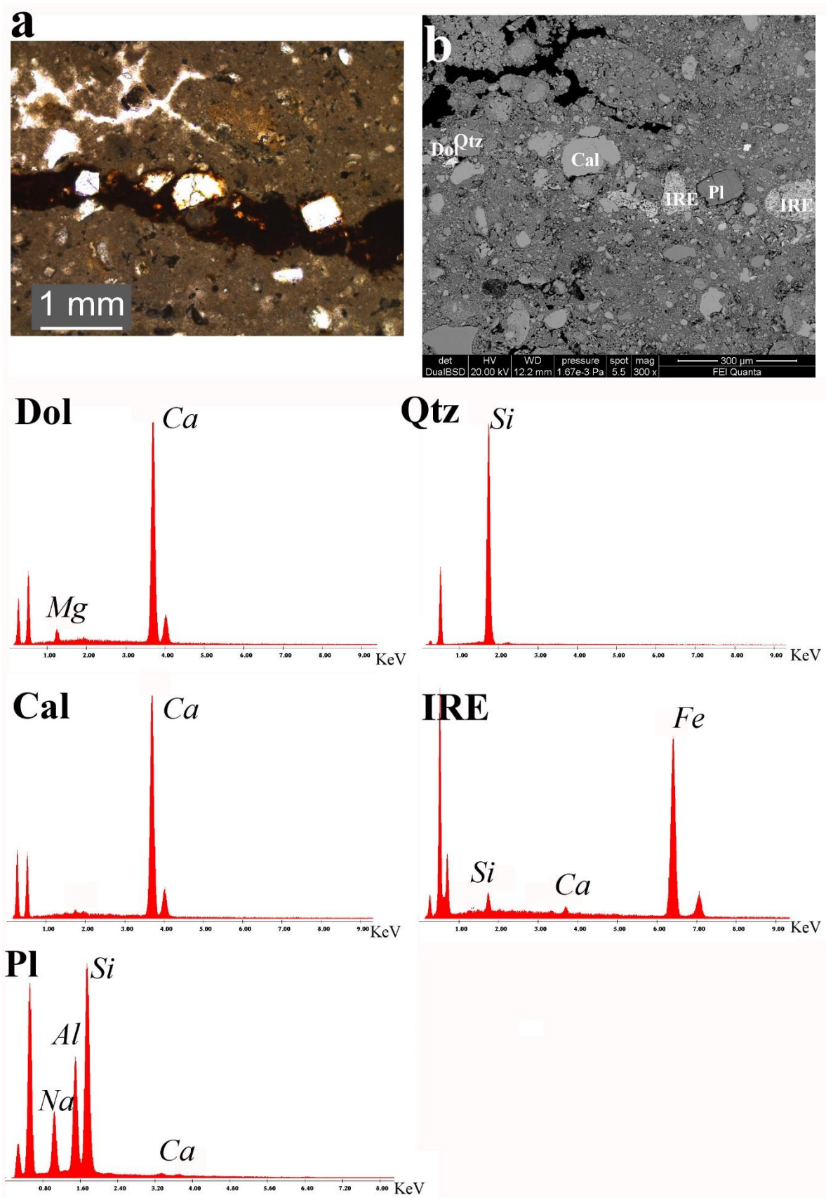
Figure 9. (a) PLM image at PPL and (b) BSE images of the paint layer (sample D7(3) A1469 M3 VII 2018/257), and EDS spectra of dolomite (Dol), quartz (Qtz), calcite (Cal), iron rich earth pigment (IRE), and plagioclase (Pl).
