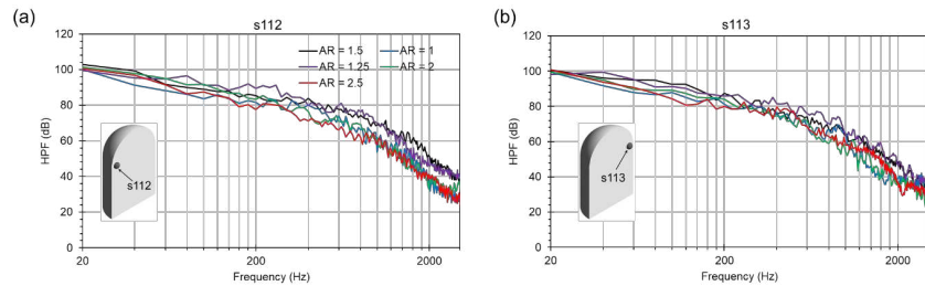
Fig. 17. Comparison of the hydrodynamic pressure fluctuations extracted on the mirror at a) s112 and b) s113 between AR = 1, 1.25, 1.5, 2 and 2.5 . The location of the sensors is indicated within each figure.
