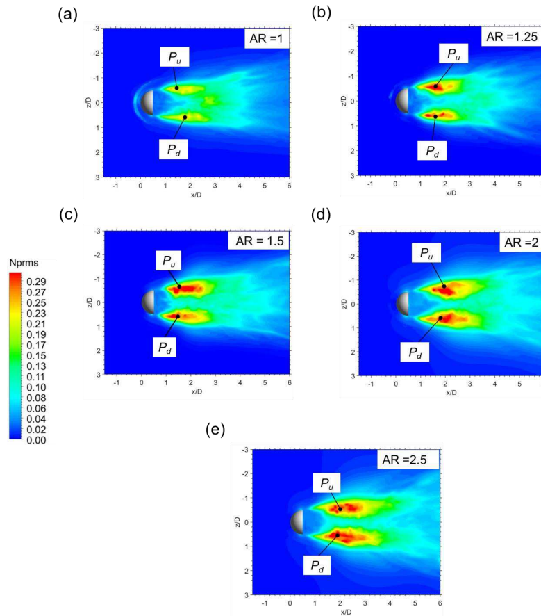
Fig. 16. Comparison of the normalised pressure fluctuations on the plate between a) AR = 1 , b) AR = 1.25 , c) AR = 1.5 , d) AR = 2 and e) AR = 2.5 . Here, P_u and P_d indicate the pressure regions formed due to the interaction of the lateral vortices with the plate.
