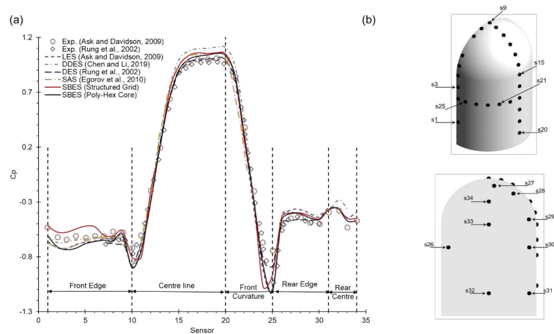
Fig. 6. a) Comparing the time-averaged pressure coefficient ( c_p ) on the surface of the mirror generated at 34 sensors is compared against experimental data 14,16 and published numerical results 14,16,21,28 and b) a schematic of the HRM with all the 34 sensors used to measure the pressure coefficient (Ref: Table 8 in Appendix A for the cartesian coordinates of the sensor locations).
