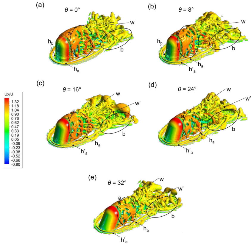
Fig. 25. Comparison of the vortical structures of an instantaneous flow field visualised by iso-surfaces of Q = 10^3 s^{-2} coloured with instantaneous x-velocity between all the sweep angles investigated: a) \theta = 0^\circ , b) \theta = 8^\circ , c) \theta = 16^\circ , d) \theta = 24^\circ , and e) \theta = 32^\circ .
