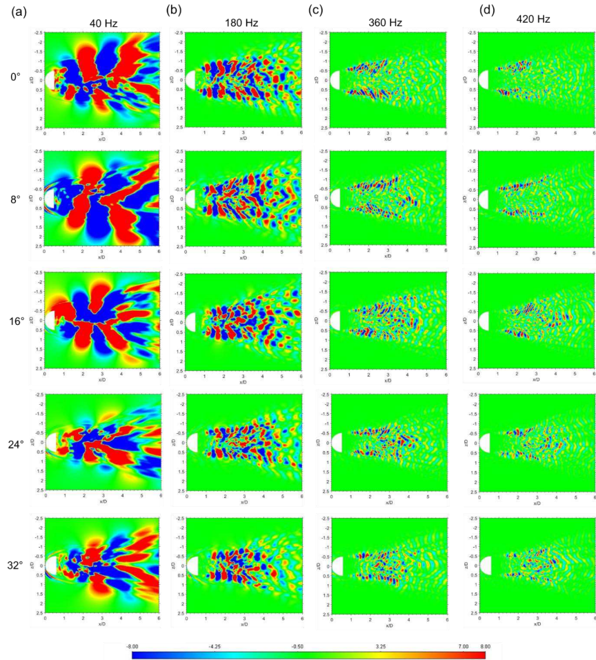
Fig. 30. Comparison of the real part of the Hydrodynamic Pressure Spectra (HPS) generated on the plate for all the sweep angles investigated, viz., 0°, 8°, 16°, 24° and 32° at a) 40 Hz, b) 180 Hz, c) 360 Hz, and d) 420 Hz.
