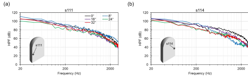
Fig. 27. Comparison of the hydrodynamic pressure fluctuations extracted on the mirror at a) s111 and b) s114 for all the sweep angles investigated: 0°, 8°, 16°, 24° and 32°. The location of the sensors is indicated within each figure.
