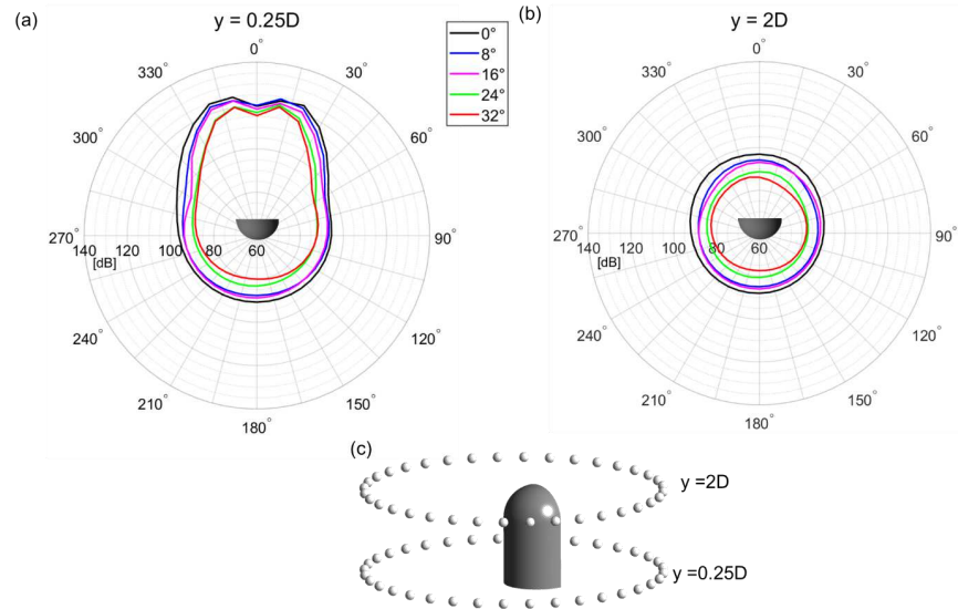
Fig. 31. Comparison of overall sound pressure level extracted at 36 microphones placed in a circular array at planes a) y = 0.25D and b) y = 2D for all the sweep angles investigated, viz., 0°, 8°, 16°, 24° and 32°, and c) illustrates the layout of the sensors located around the mirror at two different heights.
