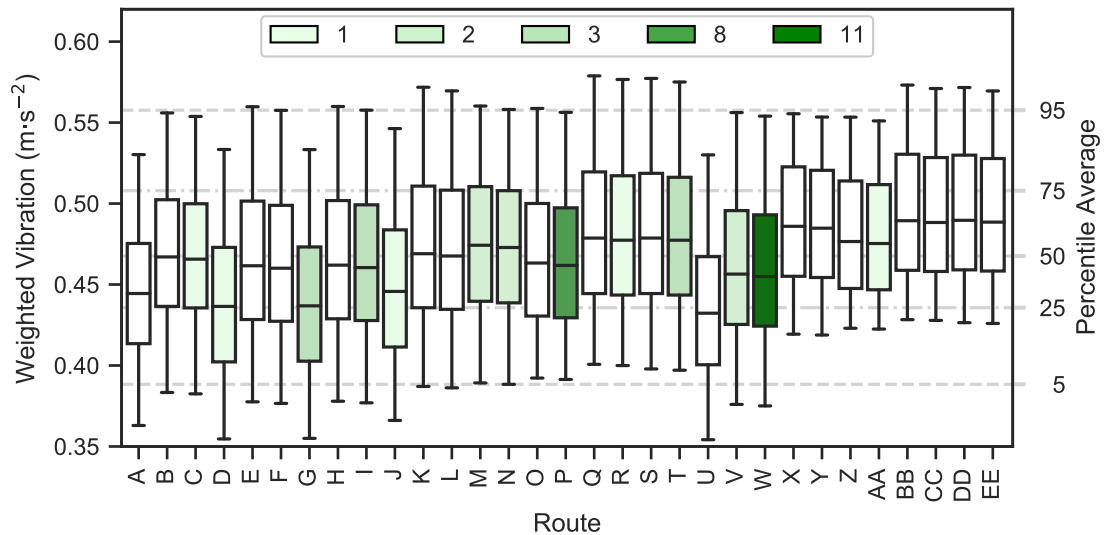
Figure 8.41: Comparison of the total combined weighted vibration for each route.
