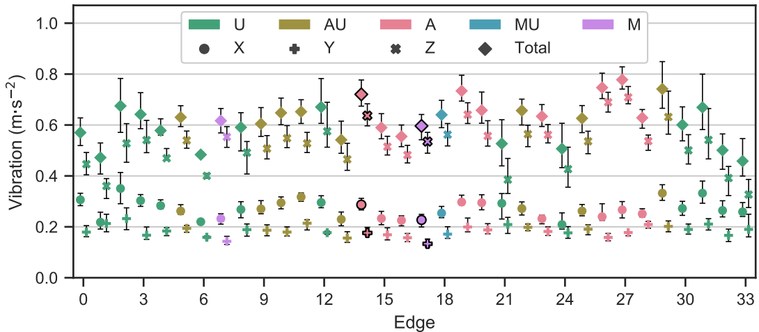
Figure 8.17: Unfiltered average vibration in each axis for each edge.
