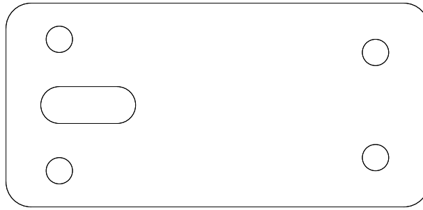
Figure 5.9: Laser-cut template used to position magnets ( \frac{1}{2} scale).
