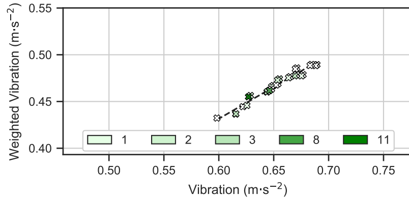
Figure 8.42: Comparison of the total comfort-weighted vibration and total un-weighted vibration for each route.
