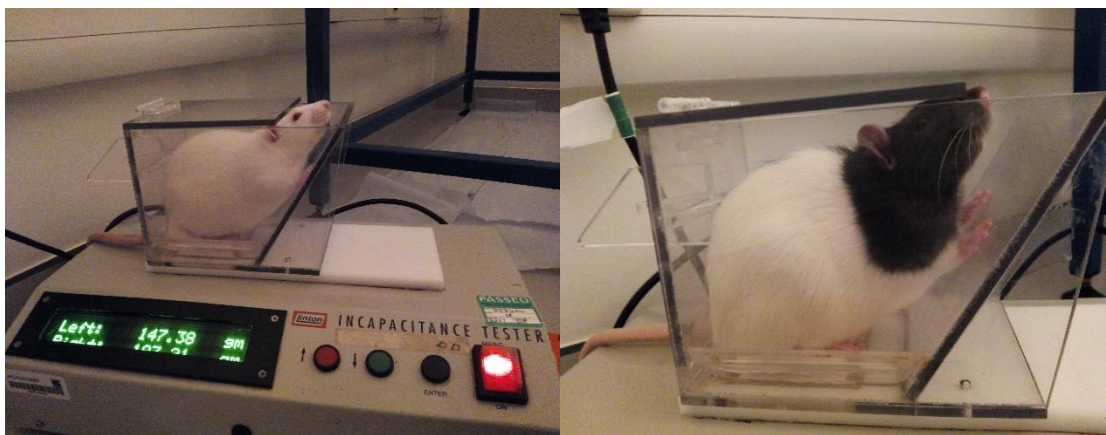
FIGURE 2.1. – INCAPITANCE METER USED FOR WEIGHT BEARING ASYMMETRY ASSESSMENTS. The incapitance meter consists in a Perspex box with a lid to hold the animal, two transducer pads in the bottom allow to record weight distributed to either hind limb by the rat. The average of the force exerted in 3 seconds was measured in grams and the collected data corresponds to the mean of three consecutive readings.
