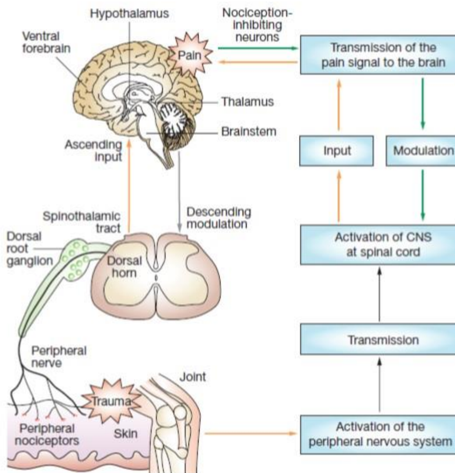
FIGURE 1.2. – PAIN PATHWAY REPRESENTATION. A peripheral activation (thermal, mechanical or chemical) is applied to the body and converted into action potentials by the nociceptor (transduction). This nociceptive information is then conducted to the dorsal horn of the spinal cord via the dorsal root ganglion (transmission). The nociceptive information is then transmitted via ascending pathways to the different supraspinal regions, where it is processed (perception). At this level, descending pathways modulate the nociceptive transmission from supraspinal areas to spinal dorsal horn (descending modulation). Image from (Bingham et al., 2009).
