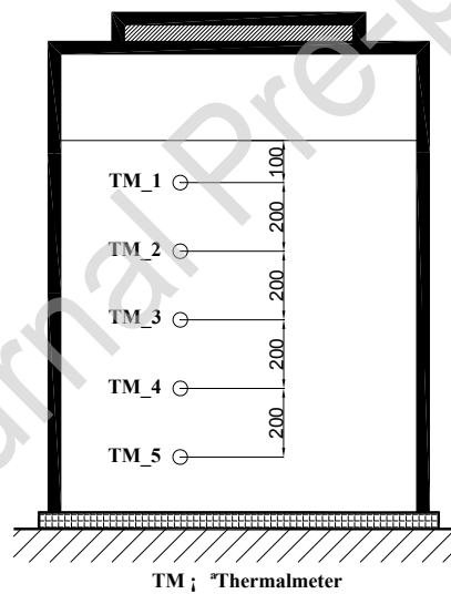
Fig.11 The distribution of the thermometers in the water tank
