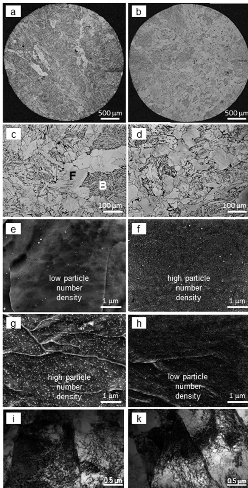
Figure 1. Optical images of the (a,b) whole samples used to measure the phase fractions and (c,d) selected areas showing ferrite-bainite microstructures (F is ferrite, B is bainite), SEM images of precipitates in (e,f) ferrite and (g,h) bainite, (i,k) TEM images of bainite for solidification rates of (a,c,e,g,i) 1 \text{ Cs}^{-1} and (b,d,f,h,k) 30 \text{ Cs}^{-1} .
