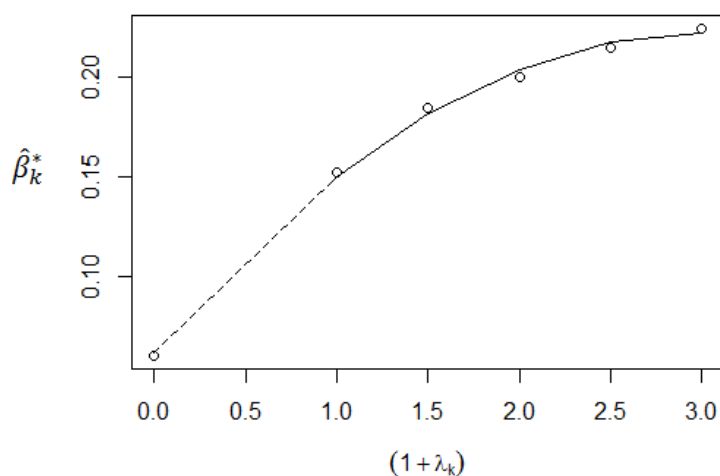
Figure 3: Extrapolation function
