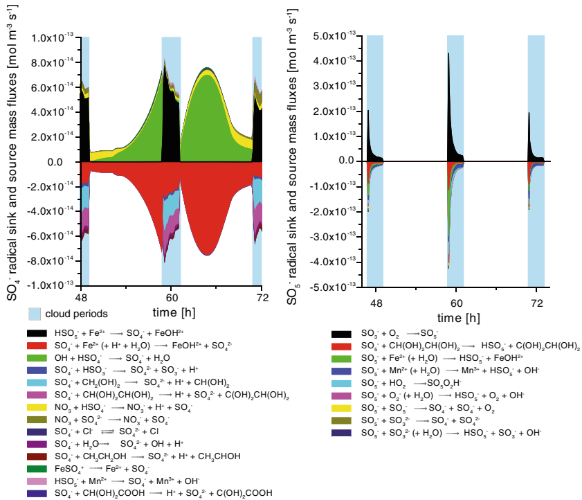
Fig. 6 Modelled aqueous chemical sink and source mass fluxes ( \text{mol m}^{-3}(\text{air}) \text{s}^{-1} ) of the \text{SO}_4^- radical (urban case, left) and \text{SO}_5^- radical (remote case, right) for a selected period of the modelling time
