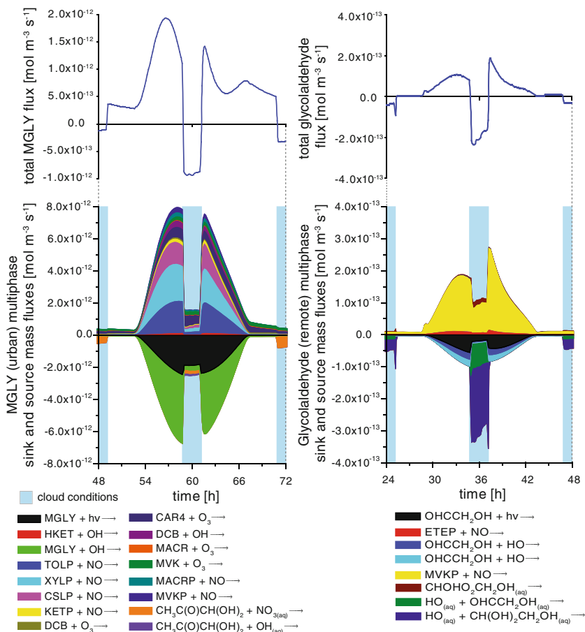
Fig. 9 Modelled multiphase chemical sink and source mass fluxes ( \text{mol m}^{-3}(\text{air}) \text{ s}^{-1} ) of methylglyoxal (MGLY, urban case, left) and glycolaldehyde (OHCC 2 H 2 OH, remote case, right) for a selected period of the modelling time
