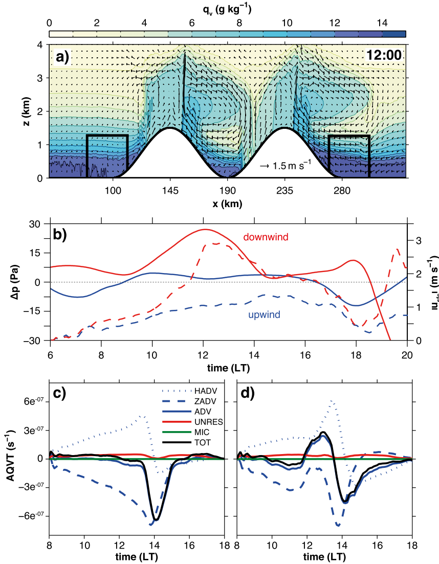
FIG. 8. (a) Vertical cross section at y = 0 \text{ km} of specific water vapor q_v (color scale) and cross-ridge wind speed (black vectors: reference vector of 1.5 \text{ m s}^{-1} ) at 1200 LT in LESd15_U30. The black boxes over the foothills downwind and upwind of the mountain sector display the control volumes used to compute the water vapor budget in Figs. 8c and 8d. (b) Time evolution of y -averaged pressure gradient between the plains (40 km away from the foothills) and the foothills (solid lines; left vertical axis) and absolute horizontal wind speed at a height of 20 m |u_{\text{stc}}| (dashed lines; right vertical axis) upwind (blue lines) and downwind (red lines) of the mountain sector. (c),(d) Time evolution of y -averaged water vapor tendencies in the (c) upwind and (d) downwind control volume depicted in Fig. 8a.
