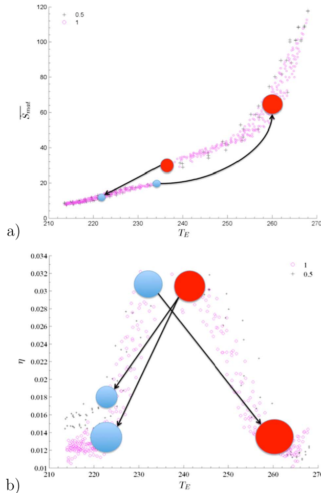
Figure 13. (a) Average rate of material entropy production ( 10^{-3} W m^{-2} K^{-1} ) versus emission temperature T_E (K) for \Omega = 0.5\Omega_{earth} (black) and for \Omega = \Omega_E (purple). (b) As in Figure 13a but for efficiency (courtesy of Robert Boschi, Universität Hamburg).
