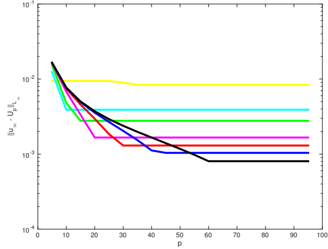
Figure 2. The error of the finite element approximation to the p -Laplacian compared to the viscosity solution to the \infty -Laplacian for various p . The colours represent different mesh refinement levels. The darker the colour, the more refined the mesh. In this experiment the meshsize ranges from h \sim 0.7 to h \sim 0.005 . Notice as the mesh is refined, best approximation is achieved for higher and higher p .
