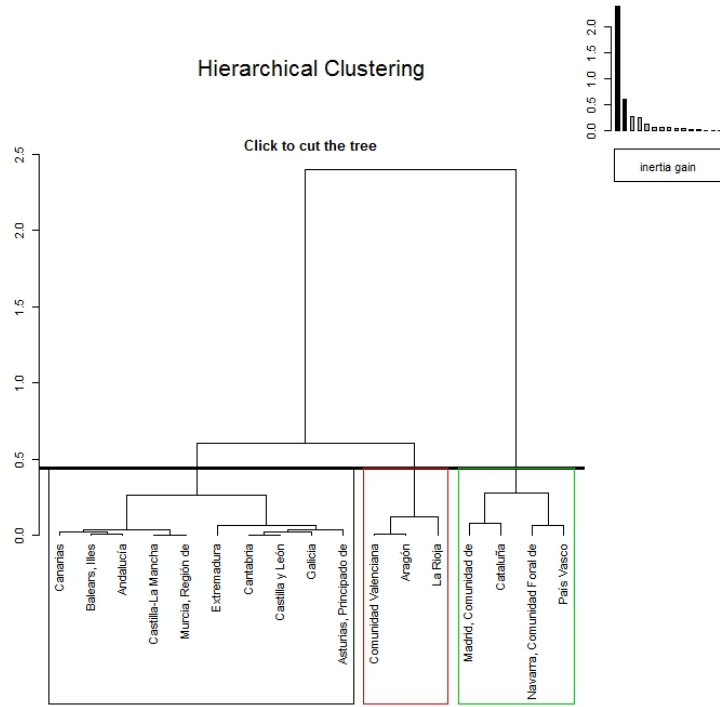
Figura 7: dendrograma cluster
