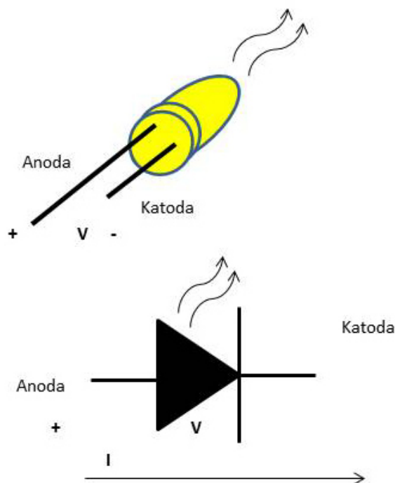
Obr. 9. LED.
