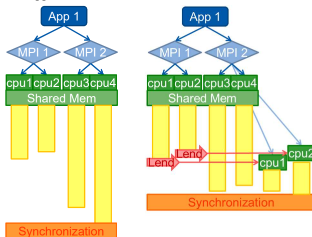
Fig. 1. LeWI Algorithm behavior: Original Application vs. Application load balanced with LeWI.
