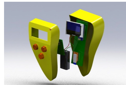
Figure 14: Exploded view of the remote and components.
