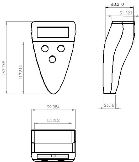
Figure 11: Dimensions of the remote
