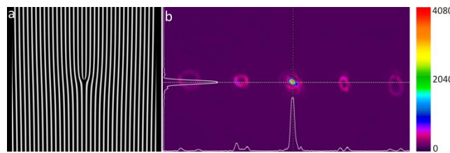
Figure 2 – a) Digital FHG for l=2 . b) Its diffraction pattern containing different LG modes. The order zero has l=0 , the first orders of diffraction are l=2 , the second ones are l=3 , etc Notice the increment of the ring radius with l .
