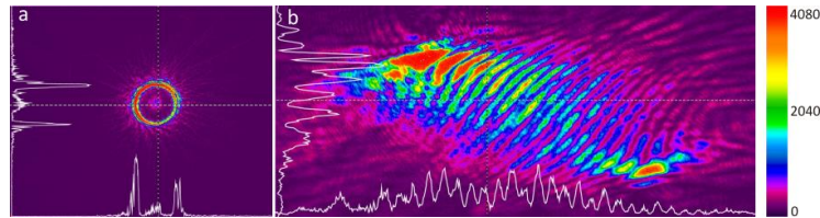
Figure 6- a) LG mode with l=20 . Cylindrical lens transformation with 20 dark fringes.
