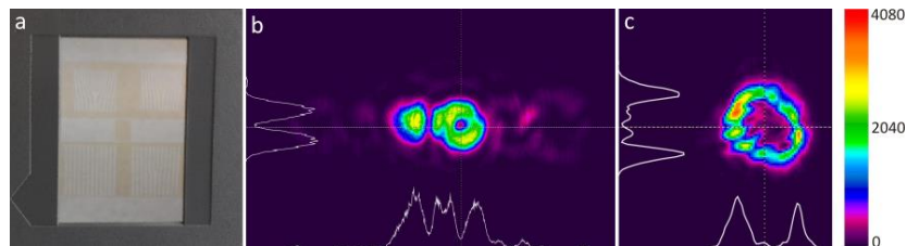
Figure 1 - a) Plate with different FHG designed for operate at 633 nm used in the laboratory b) Diffraction pattern of a FHG with l=1 at 633 nm. c) Filtered LG with l=5 generated by the correspondent FHG at 800 (note the worse quality).
