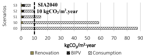
Figure 11: Global Warming Potential (kgCO 2 /m 2 .year).
