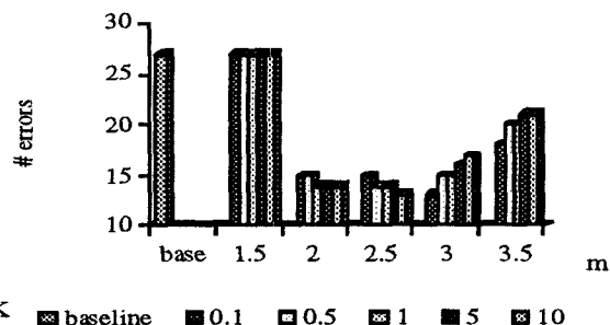
Figure 1. Recognition errors for isolated digits
