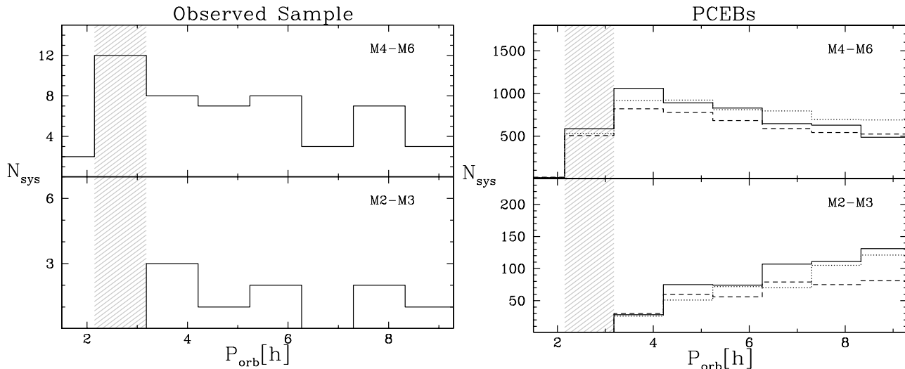
Figure 2. Left: Observed period distribution for detached WD+MS binaries. The upper and bottom panels show the distribution for different ranges of spectral types for the main-sequence companion. The corresponding ranges are labelled in the top right corner of each panel. The hatched area represents the location of the period gap (2.15 – 3.18 h, Knigge 2006). Right: Orbital period distribution for the simulated population of PCEBs with secondary stars in the corresponding spectral-type ranges. The solid line corresponds to the simulations with \alpha_{\text{CE}} = 0.25 , the dotted line to \alpha_{\text{CE}} = 0.5 , and the dashed line to \alpha_{\text{CE}} = 1.0 .
