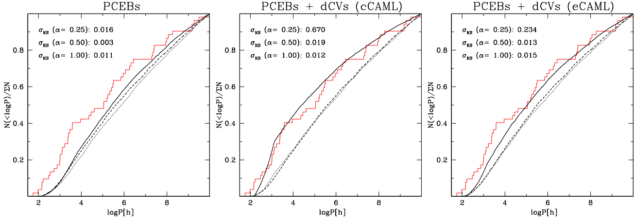
Figure 4. Comparison between the observed (red) and simulated (black) cumulative distribution of orbital periods. Left panel: only PCEBs; middle panel: PCEBs + dCVs from the cCAML model; right panel: PCEBs + dCVs from the eCAML model. The different styles of lines in each panel correspond to different CE efficiencies: \alpha_{\text{CE}} = 0.25 (solid line), \alpha_{\text{CE}} = 0.5 (dotted line) and \alpha_{\text{CE}} = 1.0 (dashed line). The values in the upper left corner of each panel are the KS probabilities.
