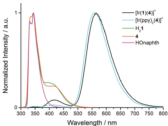
Fig. 8 Normalized solution emission spectra of [\text{Ir}(\mathbf{1})(\mathbf{4})]^+ , [\text{Ir}(\text{ppy})_2(\mathbf{4})]^+ , \text{H}_2\mathbf{1} , HO-naphth and \mathbf{4} in \text{CH}_2\text{Cl}_2 ( \sim 1.00 \times 10^{-5} mol \text{L}^{-1} ). Compounds were excited at 280 nm.
