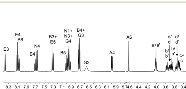
Fig. 2 The aromatic and alkyl regions of the 500 MHz 1 H NMR spectrum of [Ir(1)(2)][PF 6 ] in CD 2 Cl 2 ; scale δ/ppm. See Scheme 2 for atom labels.
