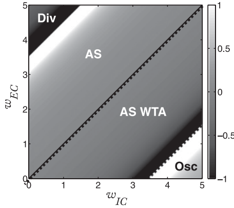
Figure 3: Stability and competitive parameter regimes for the two-column model. Shown is the derivative \partial \bar{x}_{E2} / \partial t_1 , the net effect on column 2 for an increase in the input to column 1. Competition is possible when the derivative is negative (indicated within dashed boundaries). This condition is satisfied when the mutual inhibitory coupling w_{IC} is stronger than the mutual excitatory coupling w_{EC} . Shown is the Part[11] derivative; the parameter regimes that ensure competition for Part[10] are identical, but the shape of the derivative surface is linear. Div: BIBO unstable (divergent); AS: Asymptotically stable, no competition; AS WTA: asymptotically stable, competitive regime; Osc: oscillatory dynamics caused by overly strong inhibition. w_{ER} = 2.5 ; w_{IR} = 5 . Other parameters are not relevant for the presence of competition.
