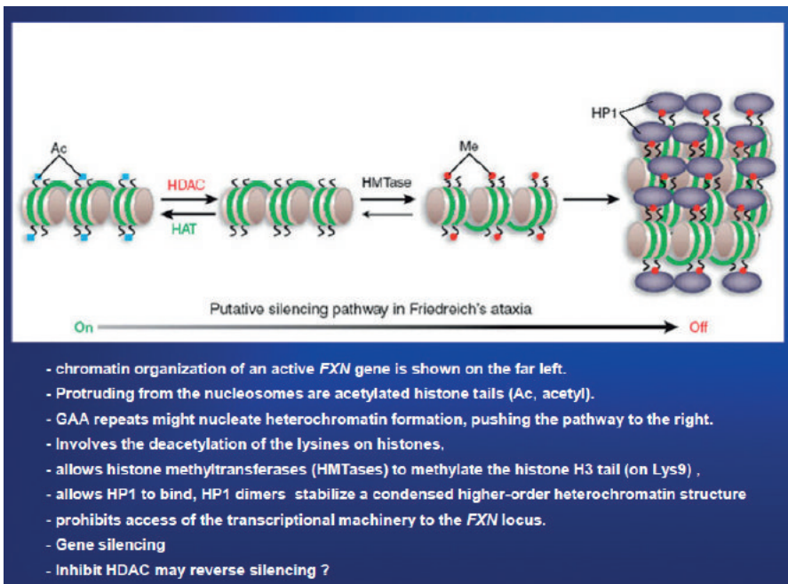
Figure 2. Putative silencing pathway in FRDA. On the far left, is an active FXN gene. Its chromatin organization consists of its DNA sequence (green) wound around nucleosomes (grey beads), consisting of octomers of the protein histone. The histones have amino-acid tails that protrude out from the nucleosomes and when they are acetylated (Ac, acetyl), an open chromatin template forms and transcription of FXN is possible. Above normal GAA repeats push the pathway to the right towards heterochromatin formation. An early step in the process of heterochromatinization is deacetylation of the lysines on the histones by HDAC (histone deacetylases). Then HMTases (histone methyltransferases) methylates histone H3 tail on its Lys9. This facilitates HP1 (purple) to bind and as nucleosomes come closer, HP1 dimers form, producing a condensed higher-order heterochromatin structure. This heterochromatinization does not allow transcription of the FXN gene. Adapted from 'Breaking the silence in Friedreich's ataxia' by Richard Festenstein.
