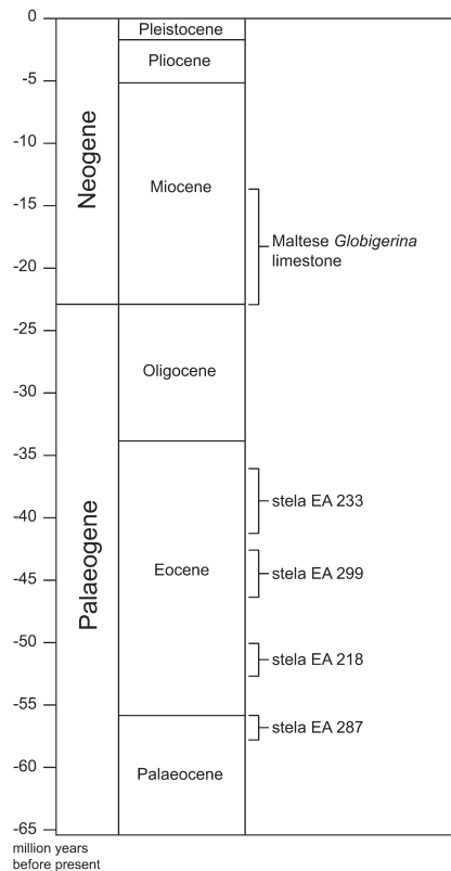
FIGURE 6. Diagram showing the relationship of the geological periods referred to in the text and the approximate ages of the stones of the stelae deduced from fossil identification and mineralogical examination
