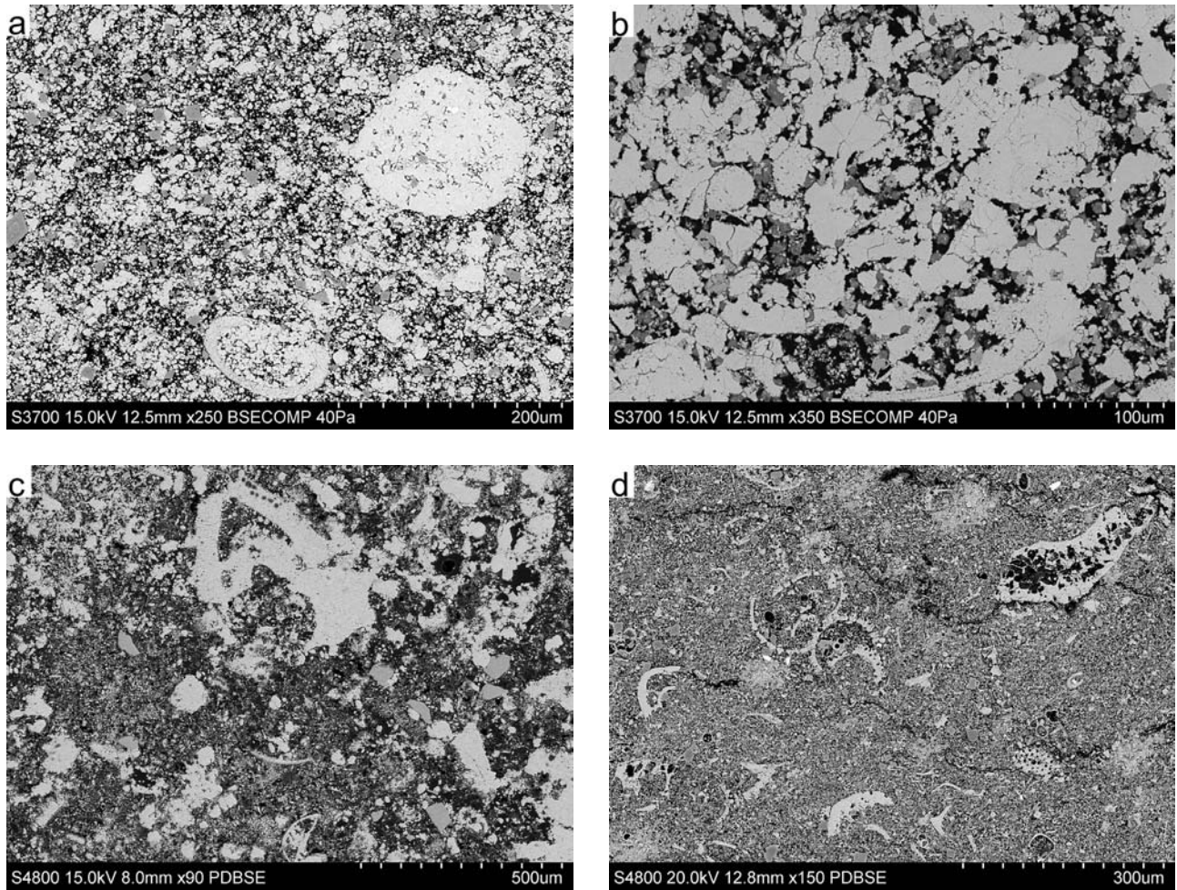
FIGURE 7. Backscattered electron images of polished thin sections of limestone samples from the four British Museum stelae: (a) EA 233; (b) EA 218; (c) EA 299; and (d) EA 287. Images: Hitachi S-3700N VP-SEM (a) and (b); Hitachi S-4800 (c) and (d)
