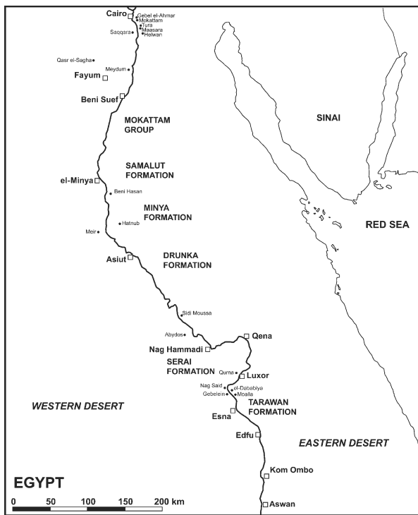
FIGURE 8. Map of Egyptian limestone formations (after [23])
