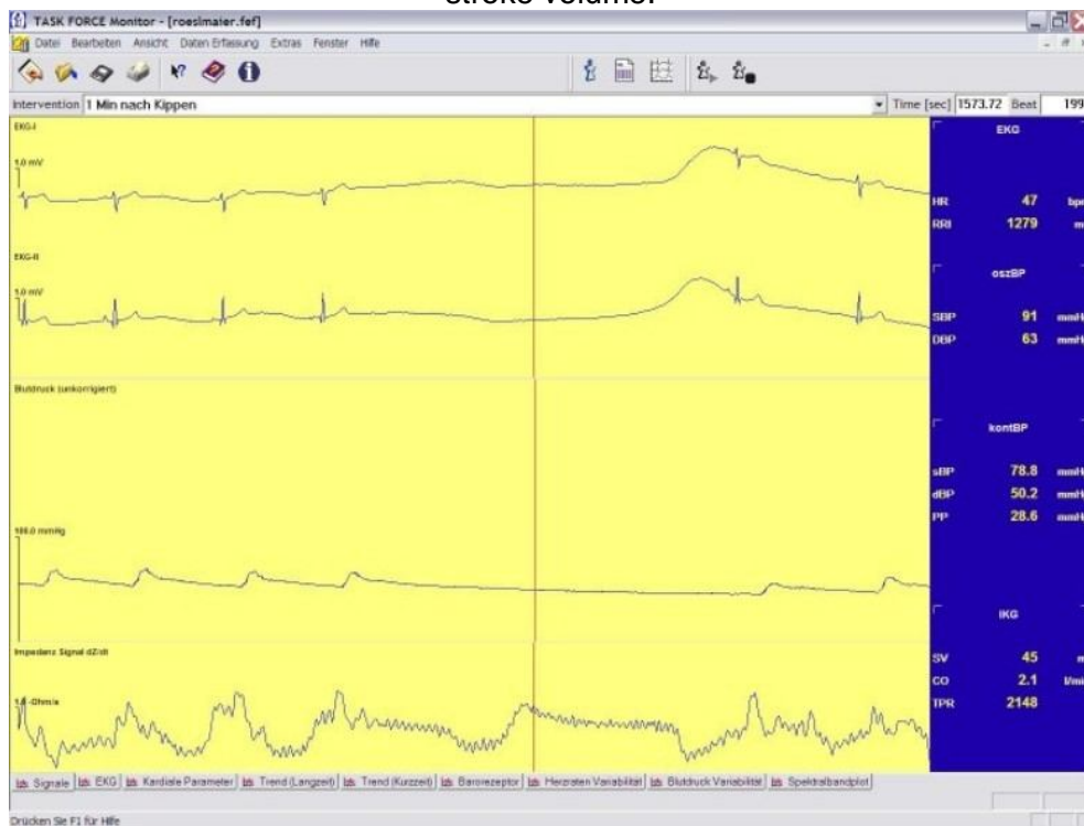
Figure 2 The same parameters during asystolia: a seven-second period without any stroke volume.
