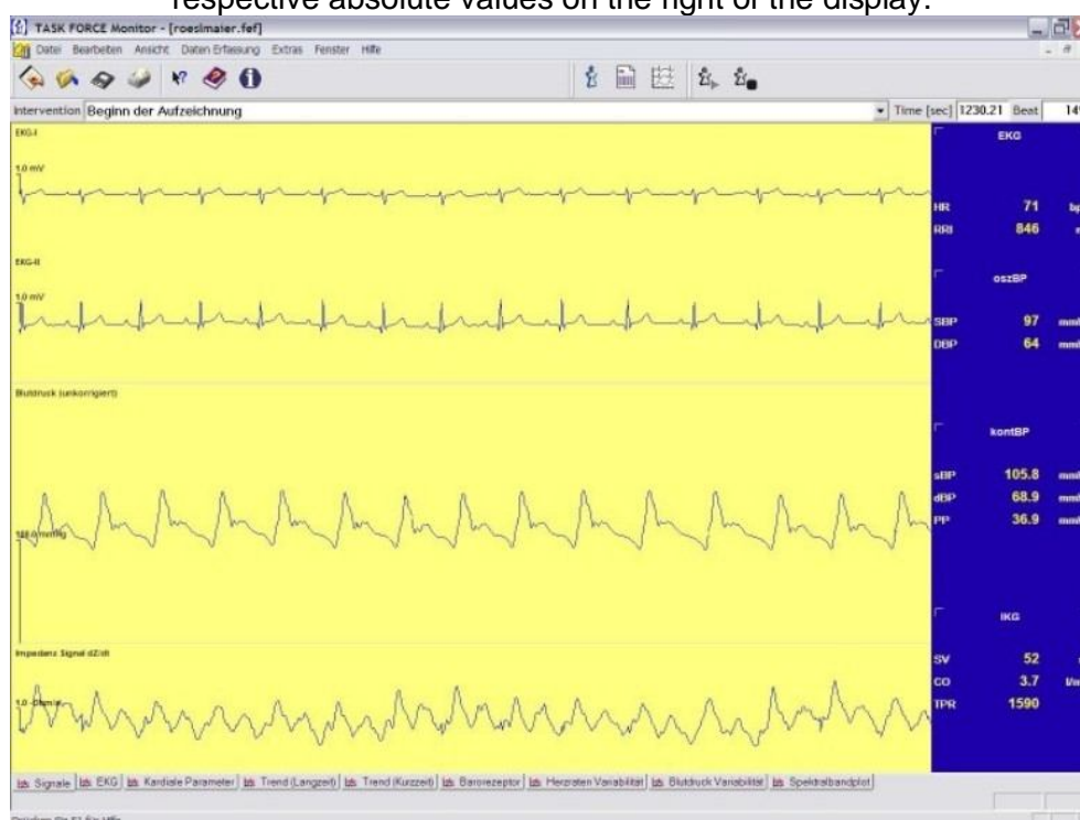
Figure 1 The patients haemodynamic parameters before tilting: two ECG tracings, the pulse-form of the beat-to-beat blood pressure and the impedance signal with their respective absolute values on the right of the display.
