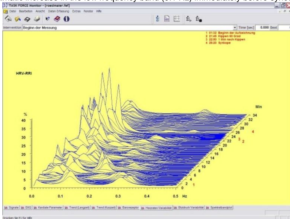
Figure 3 Power spectral analysis of heart rate variability during the test: note the dramatic increase in the low frequency band (0.1 Hz) immediately before syncope.
