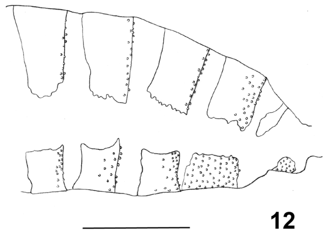
FIGURES 8–12. Asphondylia punica . 8. Head, frontal. 9. Acropod, lateral. 10. Acropod, ventral. 11. Female post-abdomen, lateral. 12. Male post-abdomen, lateral. Scale bars = 0.1 mm.
