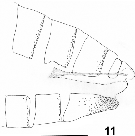
FIGURES 8–12. Asphondylia punica . 8. Head, frontal. 9. Acropod, lateral. 10. Acropod, ventral. 11. Female post-abdomen, lateral. 12. Male post-abdomen, lateral. Scale bars = 0.1 mm.
