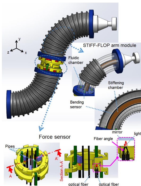
Figure 1. Overview of the STIFF-FLOP manipulator and three axis force sensor
