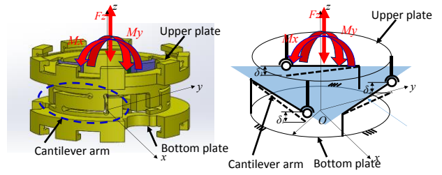
Figure 3. Equivalent spring model of the flexible tripod platform
