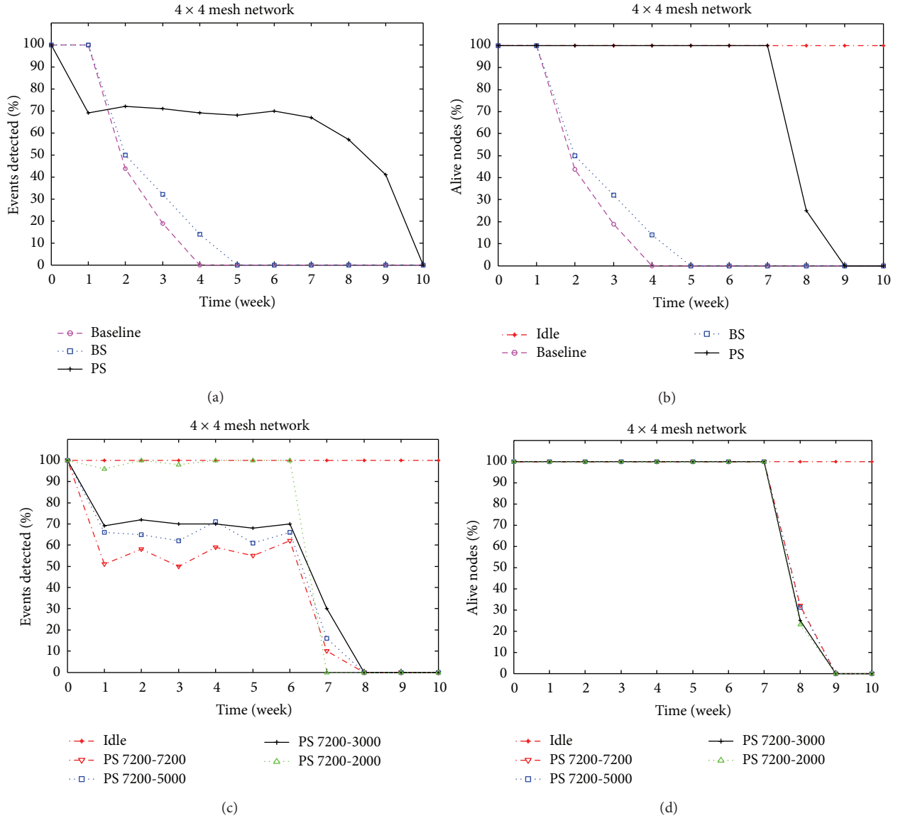
FIGURE 7: Experimental results: on 4 × 4 mesh network topology (a) % events detected, (b) % alive nodes, effects of different pheromone decay period (c) % events detected, (d) % alive nodes.
