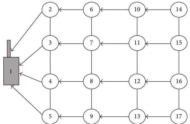
FIGURE 4: The network topology with preconfigured multihop routing chains.
