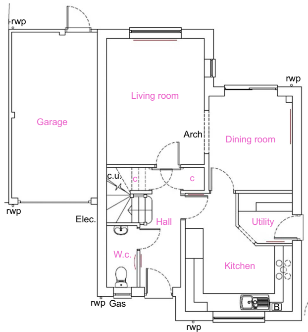
Figure 1. Ground floor plan (scale 1:50)
