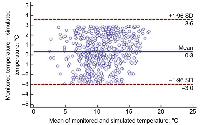
Figure 15. Bland-Altman plot outdoor temperatures (SD: standard deviation)
