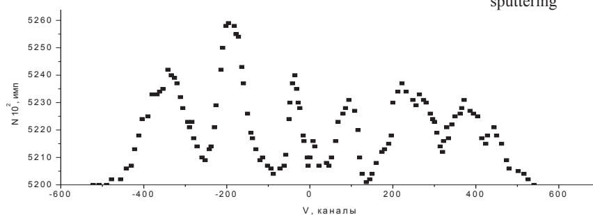
Fig. 12. CEMS spectra of \text{Bi}_{2.2}\text{Gd}_{0.8}\text{Fe}_{4.4}\text{Ga}_{0.6}\text{O}_{12} films after and annealing at 1070 K; 2.5 h
