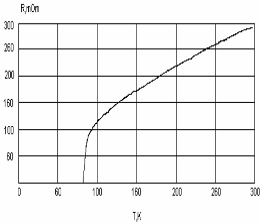
Fig. 2. The experimental temperature curve of electrical resistivity of YBa 2 Cu 3 O 7-x sample
