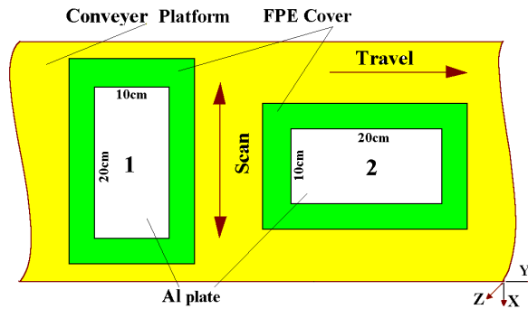
Fig. 3. Top view of two arrangements of a stack of plates with dosimetric films on moving conveyer. Position 1 - side of plates in the stack with size 20cm is oriented in direction of EB scanning. Position 2 - side of plates in the stack with size 10cm is oriented in direction of EB scanning.
