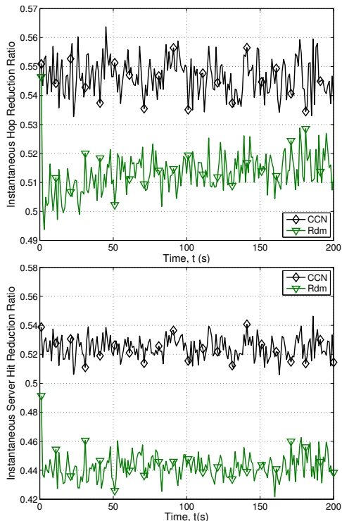
Figure 1: Simple random caching outperforming ubiquitous caching in the number of hops to hit the content (top) and reduced server hits (bottom).
