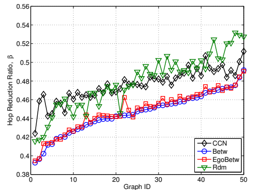
Figure 6: Performance with different B-A graphs ( N = 100 ).
