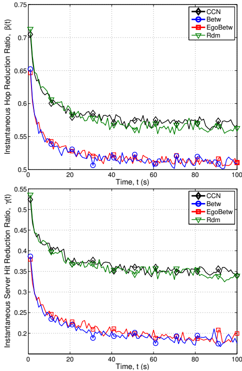
Figure 9: Instantaneous behavior of the caching schemes in a large-scale real Internet topology; (top) \beta , (bottom) \gamma .
