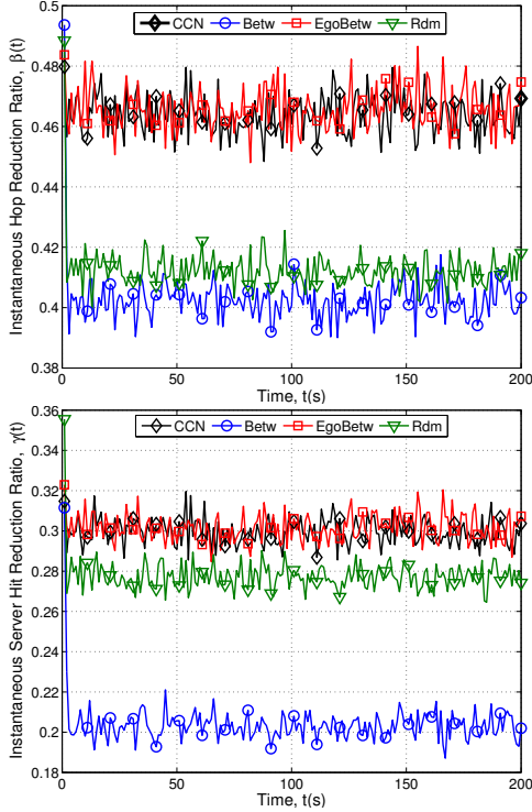
Figure 3: Instantaneous behavior of the caching schemes for a binary tree; (top) \beta , (bottom) \gamma .
