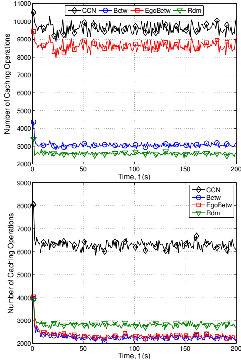
Figure 10: Number of caching operations for the different caching schemes; (top) k -ary tree, (bottom) B-A graph.
