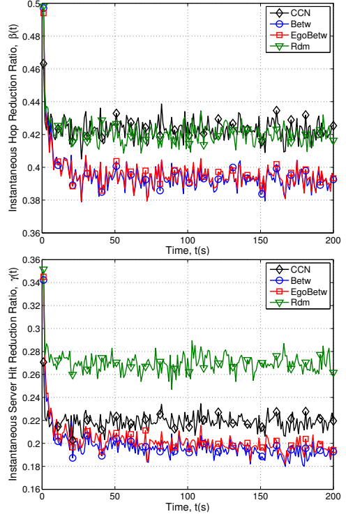
Figure 5: Instantaneous behavior of the caching schemes for a B-A graph; (top) \beta , (bottom) \gamma .
