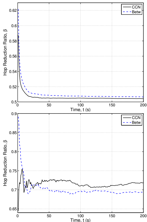
Figure 13: \beta for both weak disorder (top) and strong disorder (bottom) limits.
