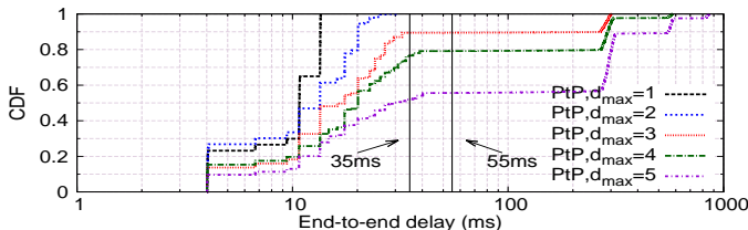
Fig. 11: End-to-end delay for the point-to-point (PtP) approach. (Color in online version.)
