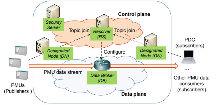
Fig. 2: C-DAX Architecture.
