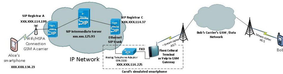
Fig. 6. The testbed environment
