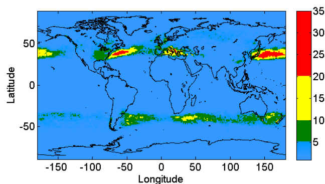
Figure 1. Global winter lightning map (color scale indicates number of thunderstorm days during the non-convective season as defined in [8]).
