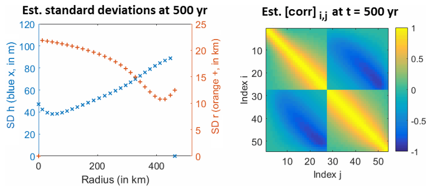
Figure 6. Standard deviations and correlation matrix Corr estimated from the 3D-Var analysis at time t = 500 years when we use only observations of ice thickness. Auto-correlations between ice thicknesses are located in the top left corner of Corr ; auto-correlations between node positions are in the bottom right corner. The rest of the matrix depicts the cross-correlations.
