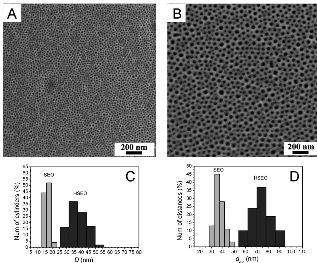
Figure 3. FESEM images of thin films ( \approx 47 nm tick) of neat samples SEO (A) and HSEO (B), prepared by spin coating toluene solutions of BCP (1.5wt%) on silicon wafers, and distribution of the values of diameters D (C) and of the center-to-center distances d_{c-c} (D) of PEO cylinders in SEO and HSEO.
