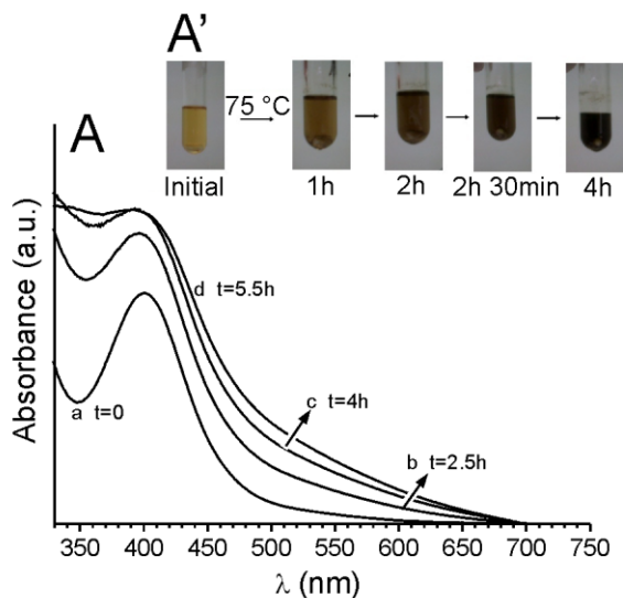
Figure 5. (A) UV-visible spectrum of a toluene solution containing HSEO (1.5 wt%) and Pd(Ac) 2 (26 wt% with respect to the BCP) (a) and of the same solution after heating at 75°C for 2.5 h (b), 4 h (c) and 5.5 h (d). 2 mL of toluene have been added to 1 mL of the initial solution before recording the UV-Vis spectra. A') Photographs of the toluene solution containing HSEO and Pd(Ac) 2 during heating at 75 °C for the indicated times.
