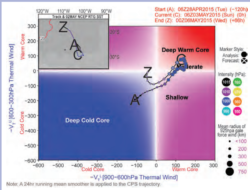
FIG. SB4.4. System phase diagram for 3 May 2015 at 0600 UTC.
