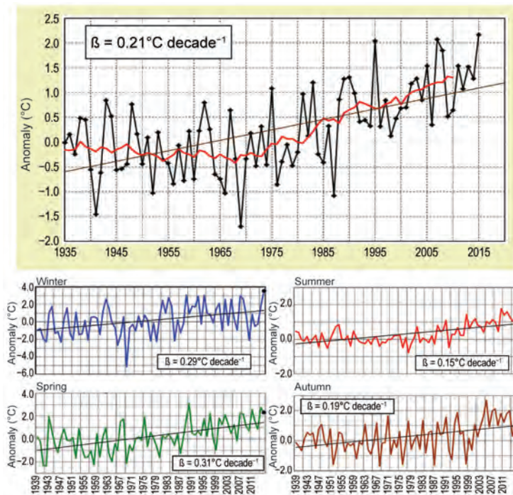
FIG. 7.43. Mean annual (1935–2015) and seasonal (1939–2015) air temperature anomalies ( ^{\circ}\text{C} ) averaged over the Russian territory for 1939–2015 (base period: 1961–90). Seasons are Dec–Feb (winter) 2014/15 and Mar–May (spring), Jun–Aug (summer), and Sep–Nov (autumn) 2015. The smoothed annual mean time series (11-point binomial filter) is shown in red in the top panel.
