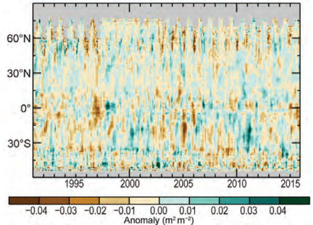
FIG. 2.27. Time–latitude diagram of soil moisture anomalies (base period: 1991–2014). Data were masked as missing where retrievals are either not possible or of low quality (dense forests, frozen soil, snow, ice, etc.). (Source: ESA CCI.)
