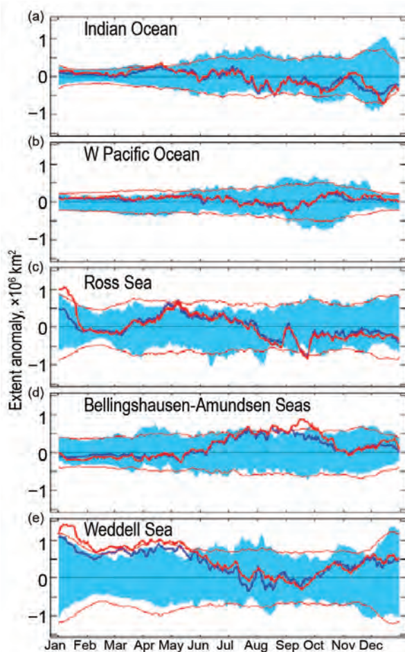
FIG. 6.9. Plots of daily anomalies ( \times 10^6 \text{ km}^2 ) from the 1981–2010 mean of daily Southern Hemisphere sea ice extent (red line) and area (blue line) for 2015 for the sectors: (a) Indian Ocean; (b) western Pacific Ocean; (c) Ross Sea; (d) Bellingshausen–Amundsen Seas; and (e) Weddell Sea. The blue banding represents the range of daily values for 1981–2010 and the thin red line represents \pm 2 std dev. Based on satellite passive-microwave ice concentration data (Cavalieri et al. 1996, updated yearly).
