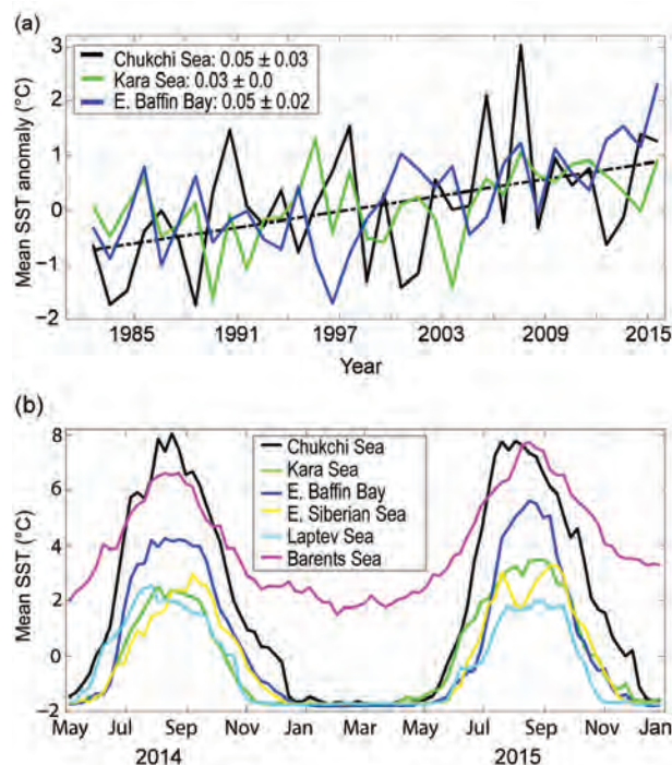
FIG. 5.8. (a) Time series of area-averaged SST anomalies ( ^{\circ}\text{C} ) for Aug of each year relative to the Aug mean for the period 1982–2010 for the Chukchi and Kara Seas and eastern Baffin Bay (see Fig. 5.7b). The dash-dotted black line shows the linear SST trend for the Chukchi Sea (the same warming trend as eastern Baffin Bay). Numbers in the legend correspond to linear trends (with 95% confidence intervals) in ^{\circ}\text{C yr}^{-1} . (b) SST ( ^{\circ}\text{C} ) in 2014–15 for each of the marginal seas, where the OISST V2 weekly product has been used in the calculation. For sea ice concentrations greater than 50%, the SST product uses a linear relationship with sea ice concentration to infer SST; variations in freezing temperature as a consequence of salinity variations imply that SSTs inferred from sea ice can be erroneously cool by as much as 0.2^{\circ}\text{C} , with the highest errors in the Canadian sector (see Timmermans and Proshutinsky 2015).
