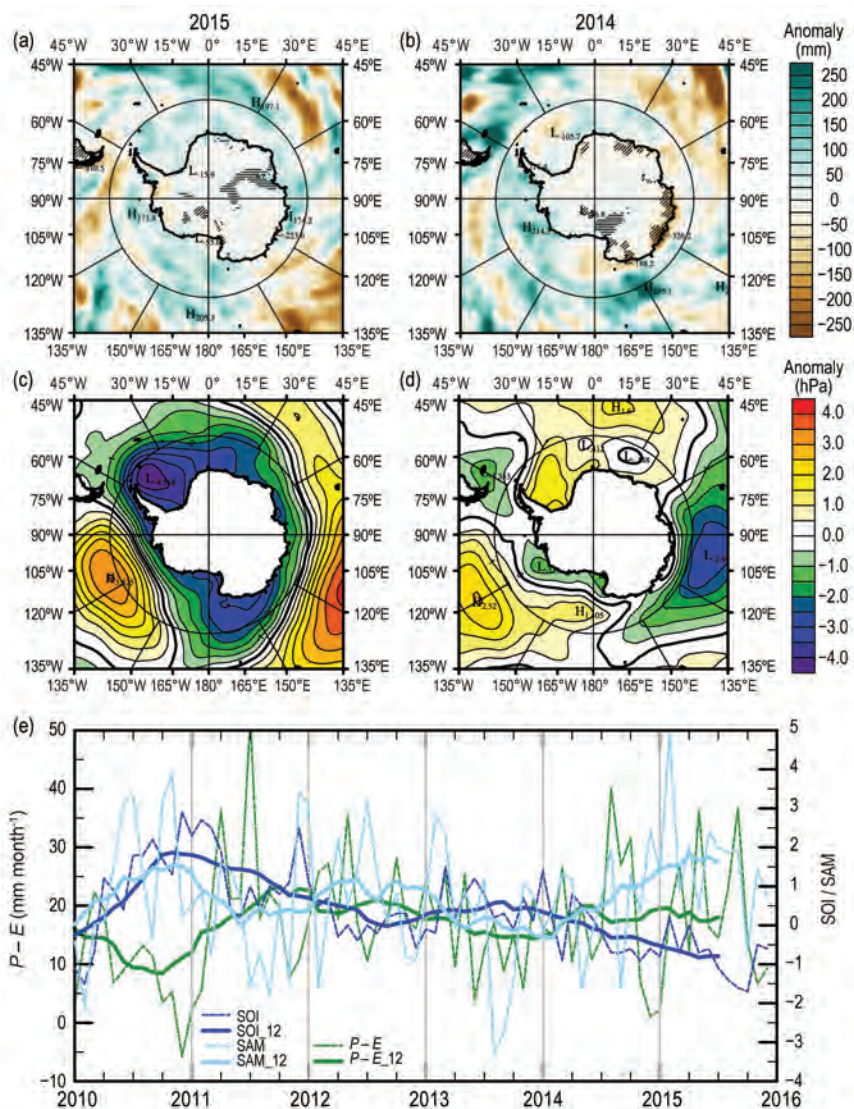
FIG. 6.5. JRA-55 (a–d) annual P-E and MSLP anomalies: (a) 2015 P-E anomalies ( \text{mm month}^{-1} ); (b) 2014 P-E anomalies ( \text{mm month}^{-1} ); (c) 2015 MSLP anomalies ( \text{hPa} ); and (d) 2014 MSLP anomalies ( \text{hPa} ). All anomalies are departures from the 1981–2010 mean. (e) Monthly total P-E ( \text{mm} ; dashed green) for the West Antarctic sector bounded by 75^\circ\text{--}90^\circ\text{S} , 120^\circ\text{W--}180^\circ , along with the SOI (dashed dark blue, from NOAA Climate Prediction Center) and SAM [dashed light blue, from Marshall (2003)] indices since 2010. In (a) and (b), Antarctic regions with greater than \pm 30\% change are hatched; sloping denotes negative values and horizontal denotes positive. Centered annual running means are plotted as solid lines.
