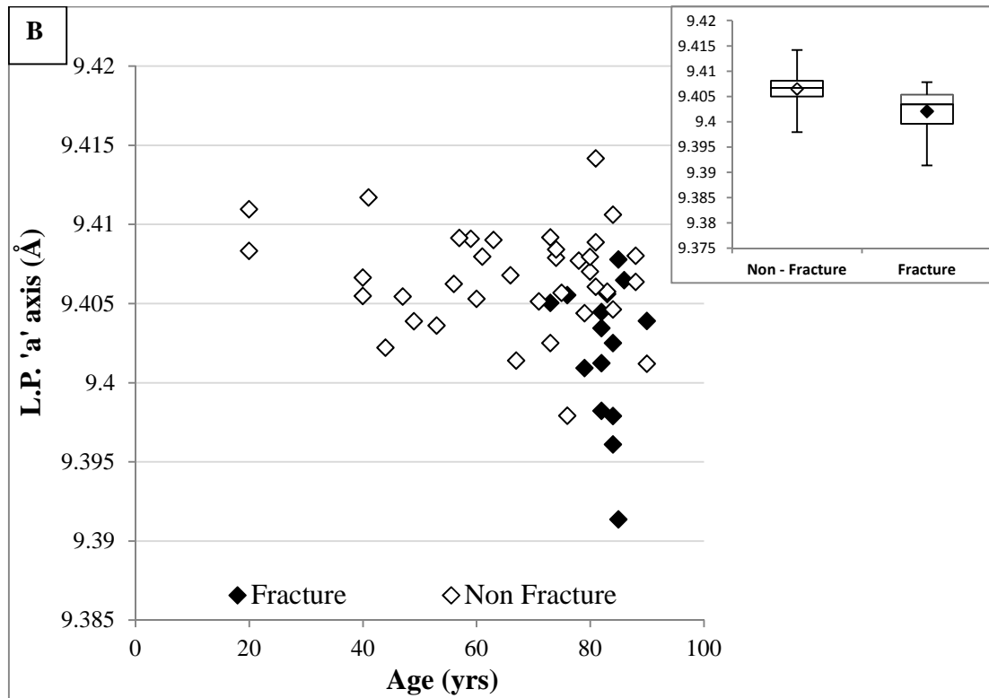
Figure 1: Relationship between XRD parameters and age (A: coherence length (CL) values along the 00\ell direction vs age, B: 'a' axis lattice parameters vs age), for fracture and non-fracture specimens. Errors have been excluded from the graphs for clarity. Standard box and whisker plots for the age matched data (70 years +) are included as inserts in each graph. The horizontal line within the box indicates the median, boundaries of the box indicate the 25 th and 75 th percentile, and the whiskers indicate the highest and lowest values of the results. The '◊' marked in the box indicates the mean.
