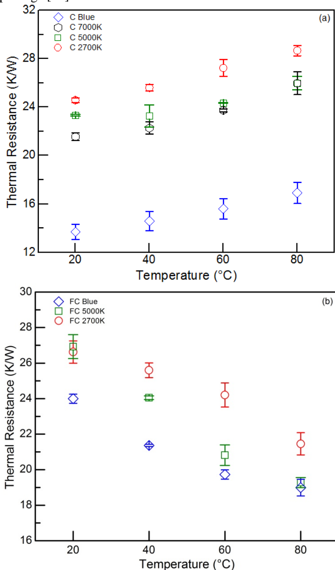
Fig. 5. Real thermal resistance of (a) conventional and (b) flip-chip bonded LEDs at different operating temperatures.
