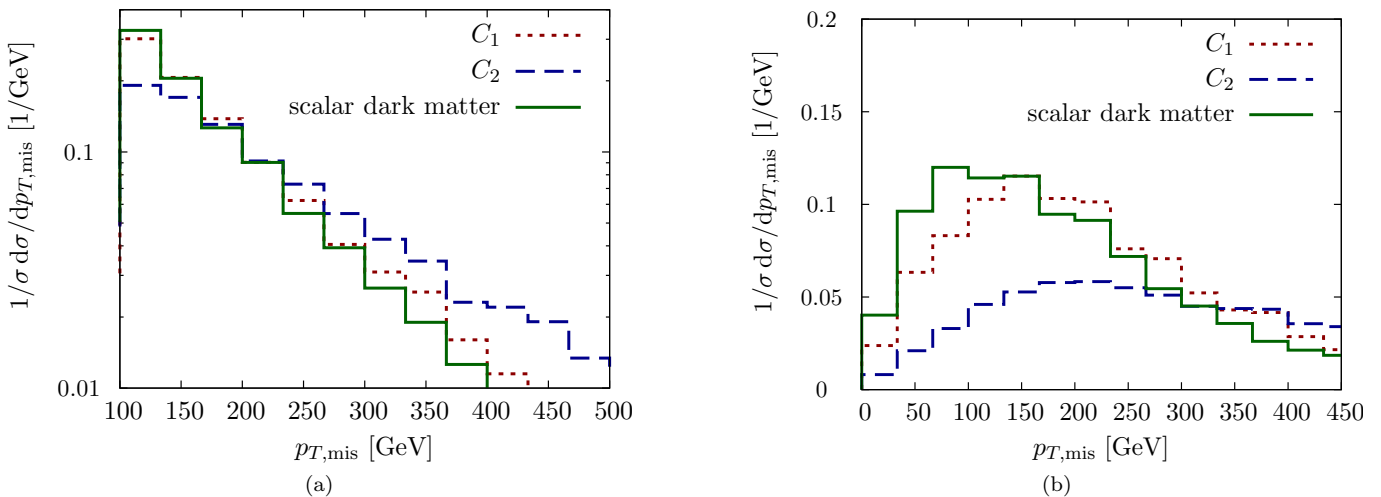
FIG. 3: Shape comparison of the dark energy scalar p_{T,\text{mis}} distribution for (a) 2\phi+\text{jet} and (b) 2\phi + t\bar{t} with a scalar mediator of mass 1 TeV. Dark energy and dark matter particle masses are chosen identical (see text), all other parameters only affect the overall normalisation of the distributions.
