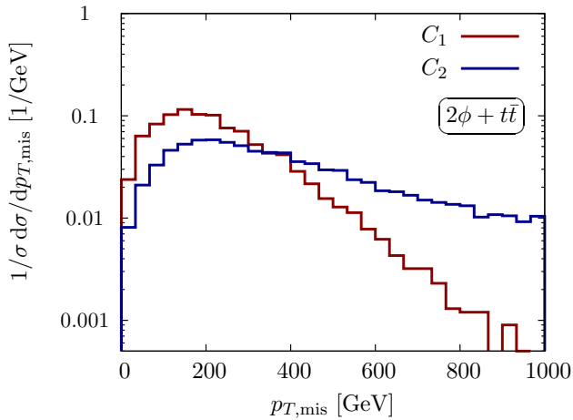
FIG. 2: Shape comparison of the t\bar{t} +transverse momentum distribution in the presence of conformal and disformal couplings, Eqs. (II.5) and (II.6).
