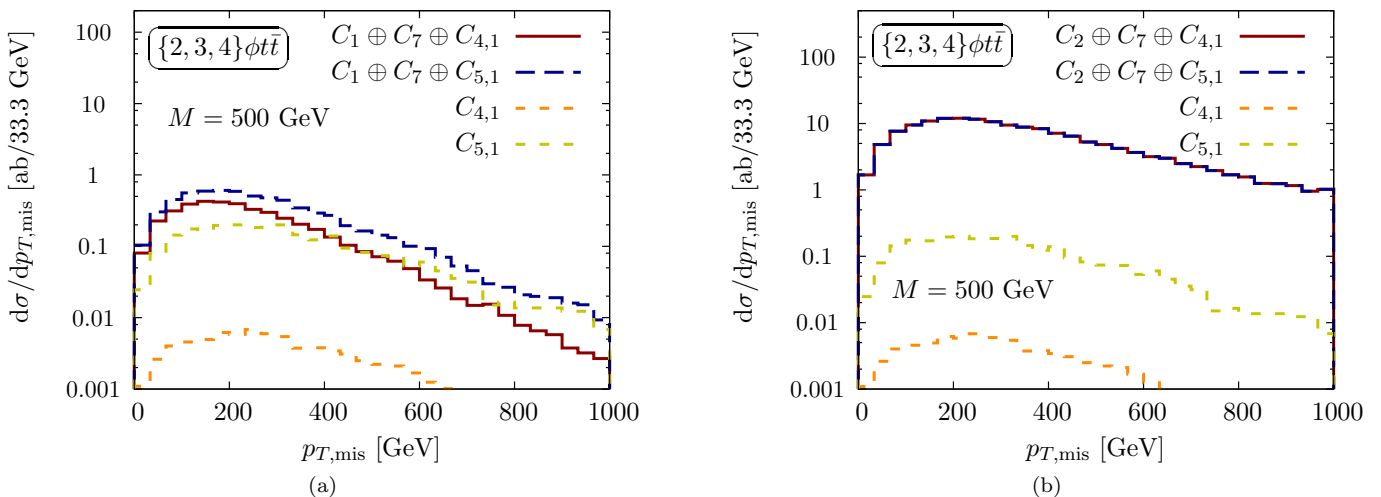
FIG. 8: Same as Fig. 6 expect that we consider the interactions parameterised by C_1 (a) and C_2 (b) for the t\bar{t} + p_{T,\text{mis}} final state for the operators C_{4,1} and C_{5,1} .
