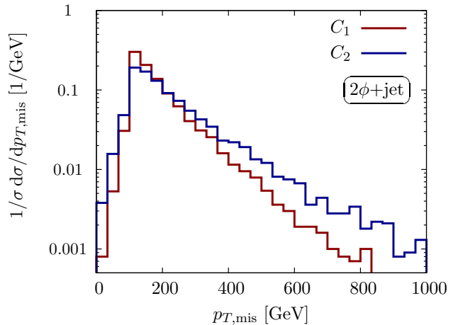
FIG. 1: Shape comparison of the jet+missing transverse momentum distribution for conformal and disformal couplings, Eqs. (II.5) and (II.6).
